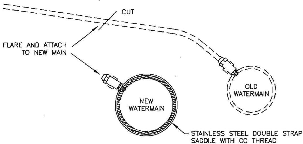
LONG SIDE TRANSFER NTS
