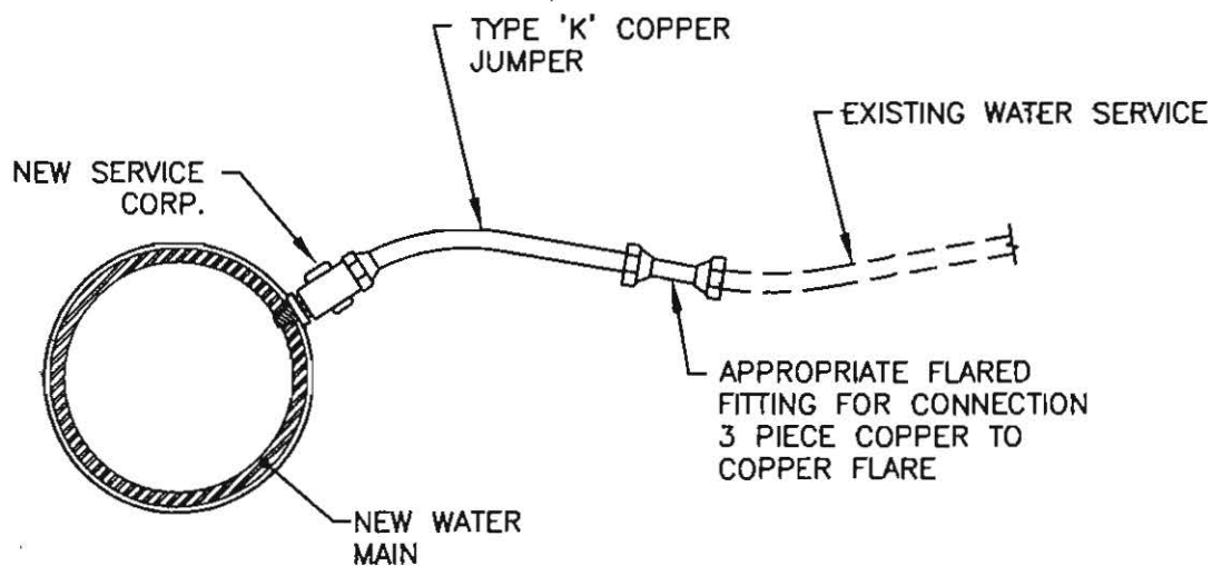
SHORT SIDE TRANSFER NTS
