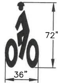
DESIGNATED BICYCLE LANE SYMBOL
