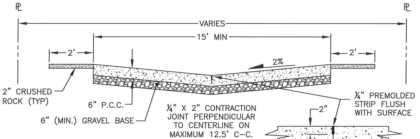
ALTERNATE B CEMENT CONCRETE ALLEY PAVEMENT
